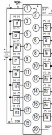
Field Wiring Terminals Field Wiring
